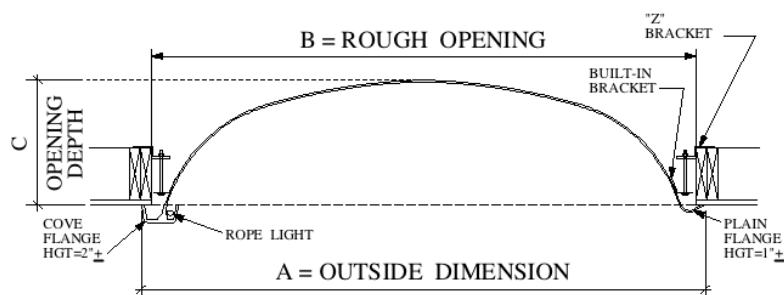
DOMES DIMENSION DIAGRAM
